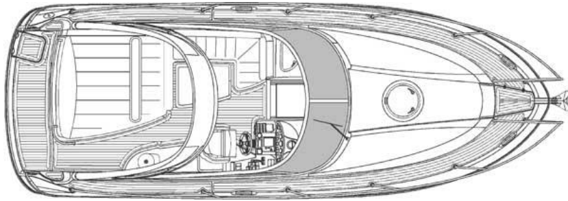
Deck Layout
