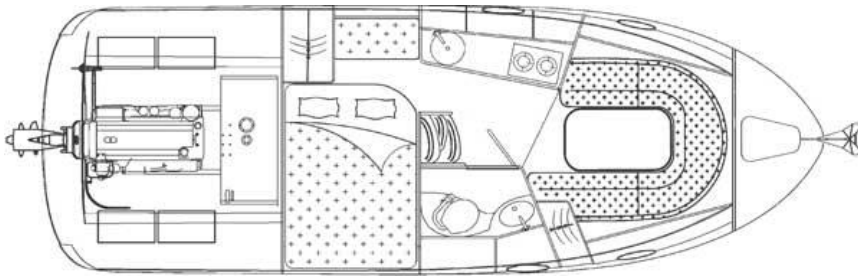
Internal Layout
