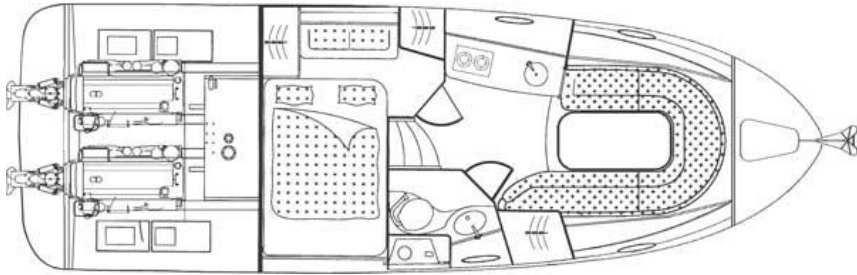
Internal Layout
