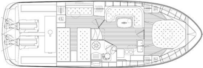
Internal Layout
