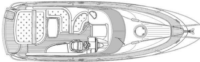
Deck Layout
