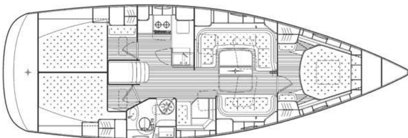
3 Cabin Layout
