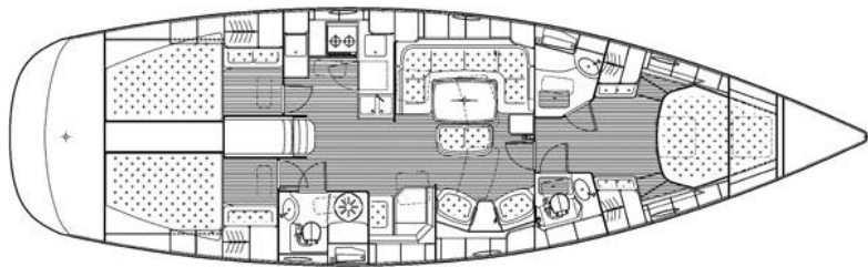
Cabin Layout
