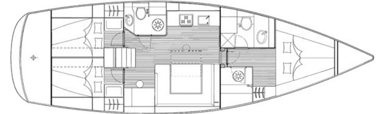
3 Cabin Layout
