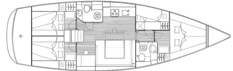
4 Cabin Layout
